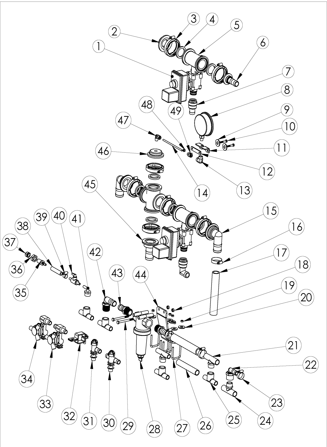
9410,9430,9500 Series Boom Plumbing
