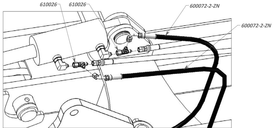
VIEW AT LATCH CYLINDER
