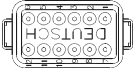
PIN OUT DETAIL
