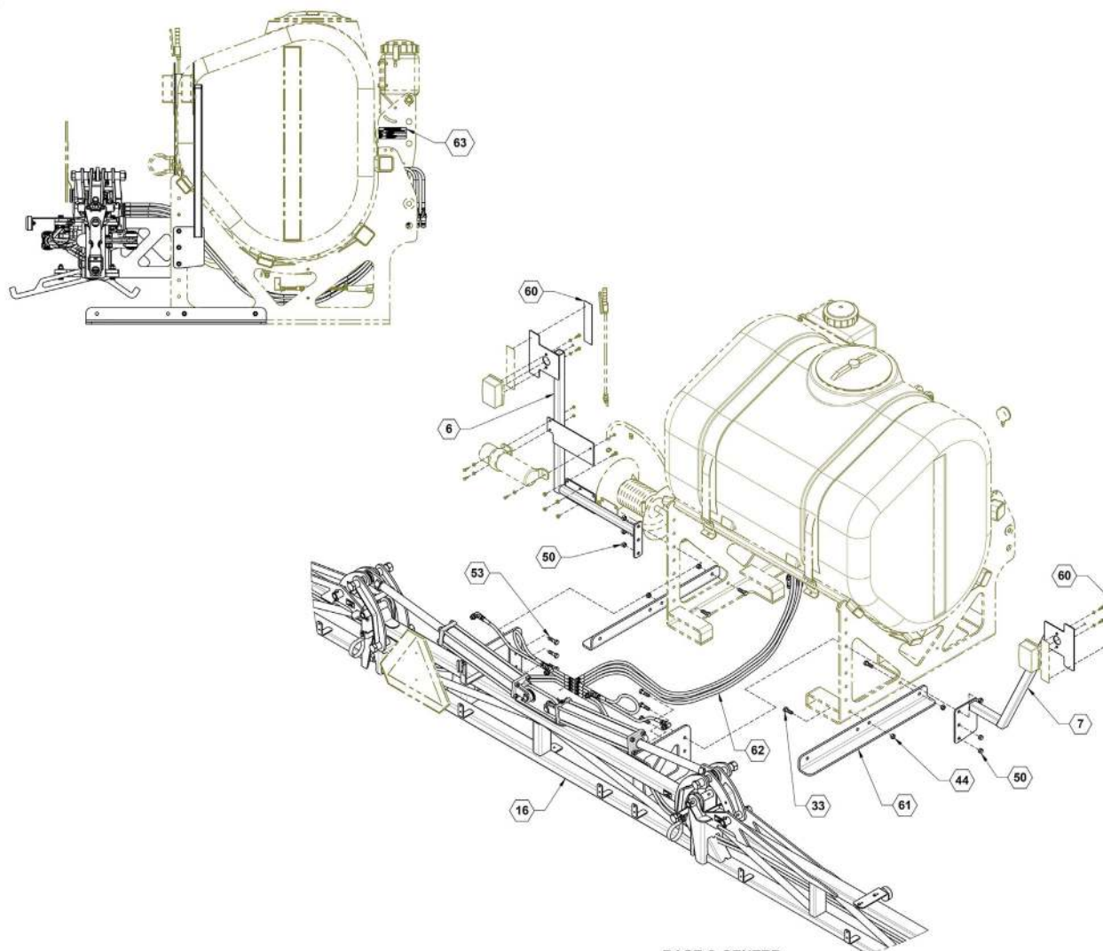
BASE & CENTER SECTION ASSEMBLY
