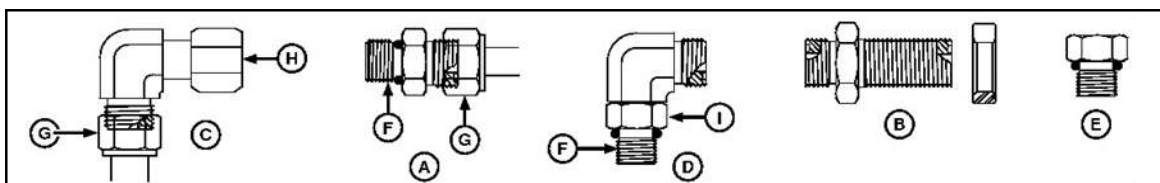
Figure 27: Common hydraulic fitting shapes and components
