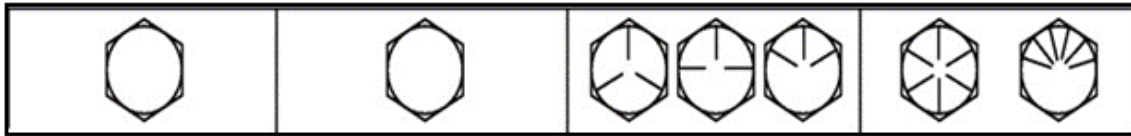
Figure 26: Common imperial bolt grade markings
