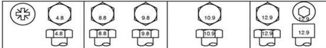
Figure 25: Common metric bolt grade markings
