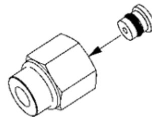
Figure 12: Restrictor Orifice
