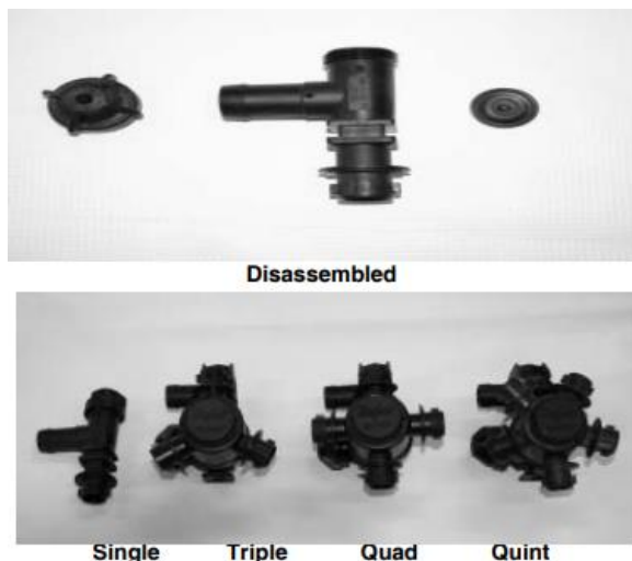
Figure 18: Nozzles typical for a dry boom
