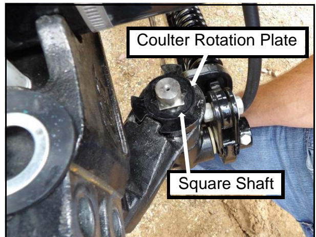
Coulters in line with mount
