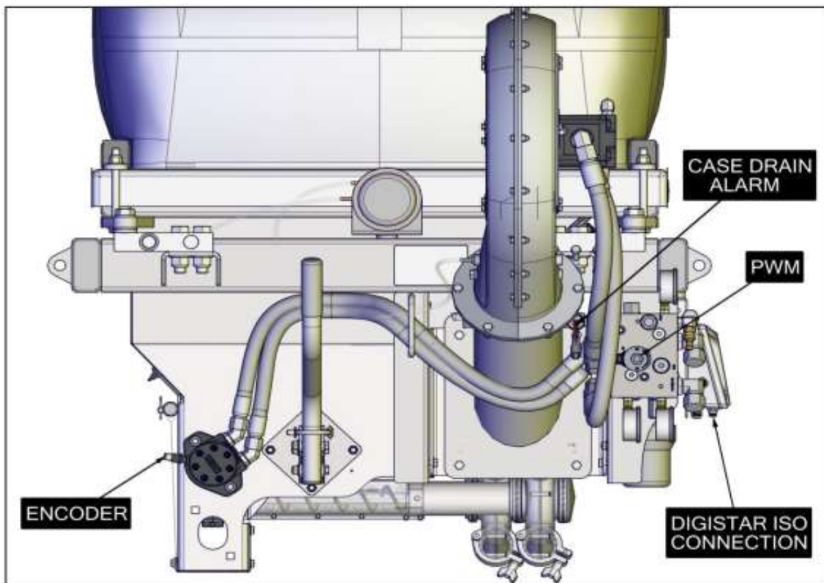
6.4 2108 HARNESS CONNECTION
