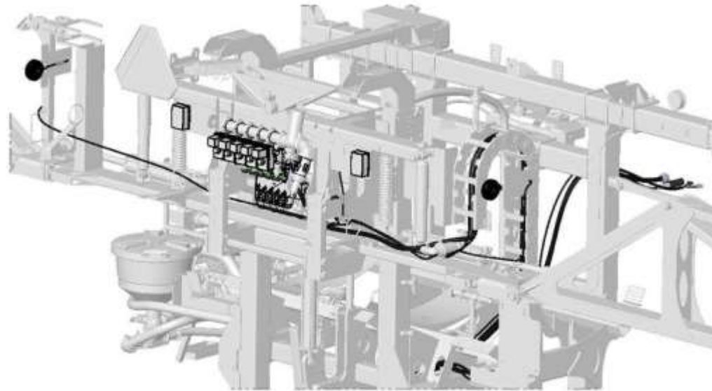
9573PTF HARNESS I.D. AND LOCATION
