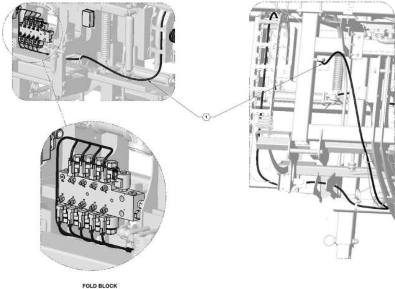
FOLD BLOCK
