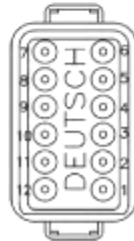
PIN OUT DETAIL FOR RECEIPT
