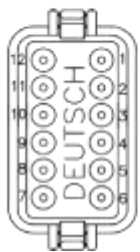
PIN OUT DETAIL FOR PLUG
