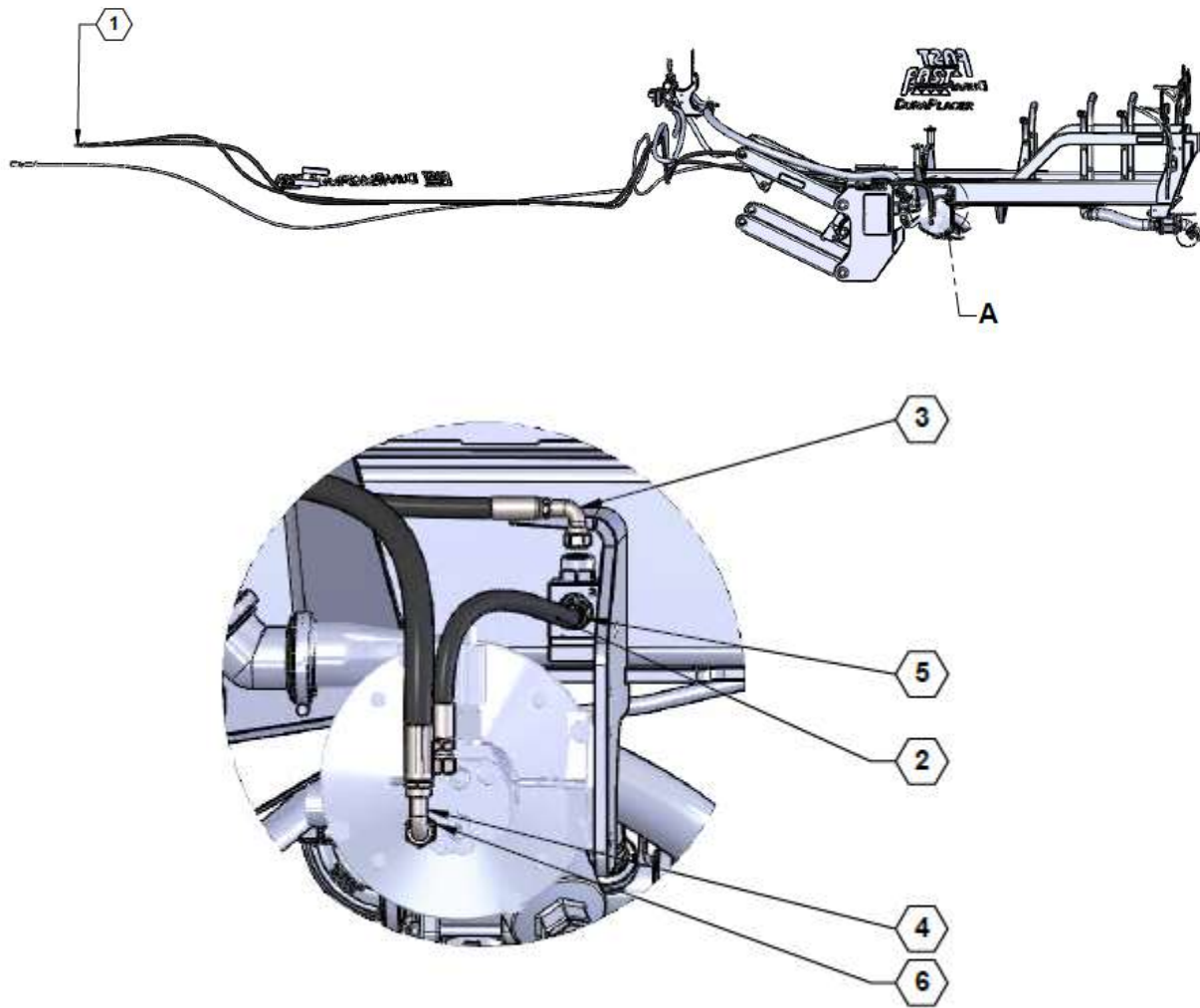
DETAIL A
