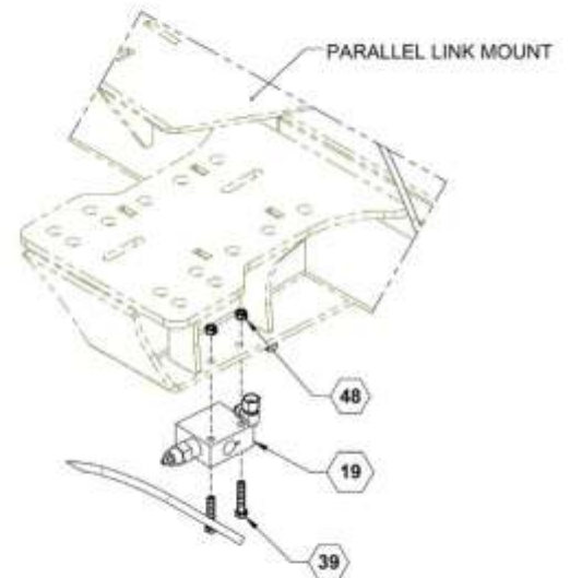
COUNTERBALANCE VALVE
