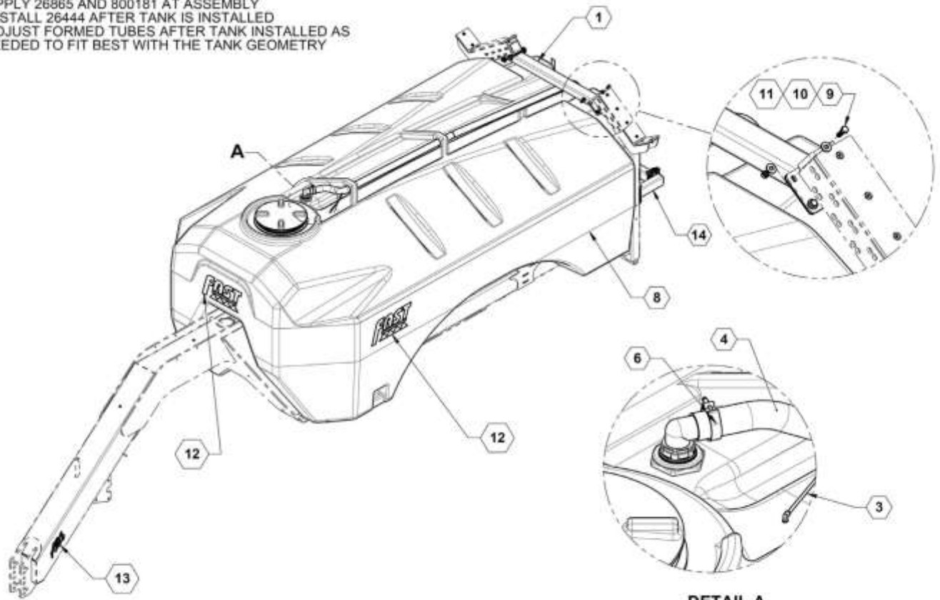
DETAIL A
