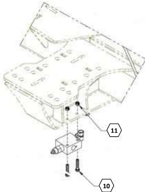
COUNTERBALANCE VALVE
