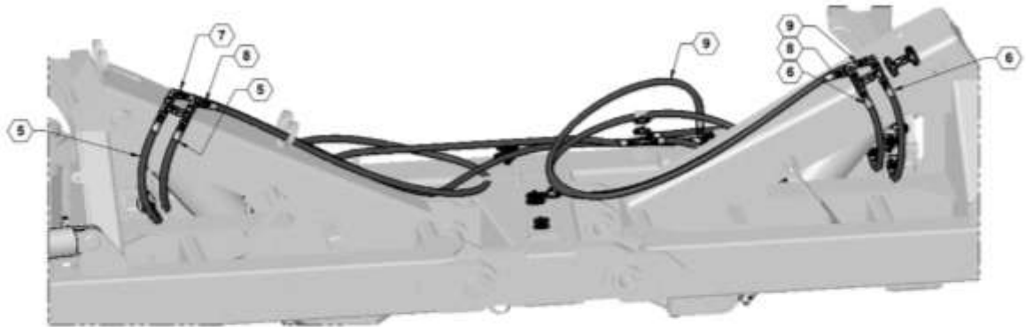
INNER WING HYDRAULIC HOSE ROUTING
