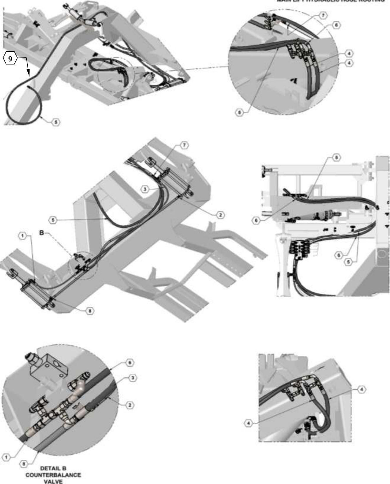
MAIN LIFT HYDRAULIC HOSE ROUTING
