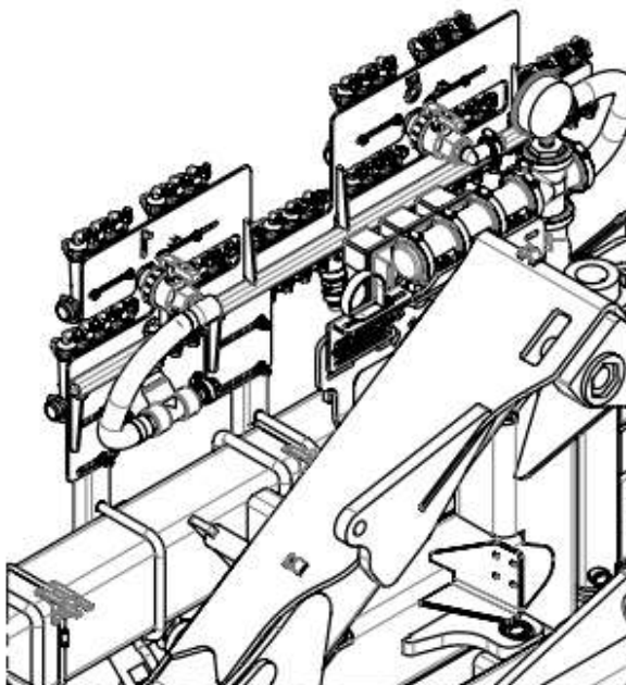
REAR VIEW OF WILGER MONITORS & ELECTRIC VALVES
