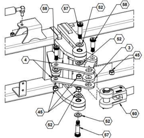
SWING WING HINGE ASSEMBLY
