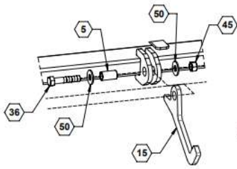
WING LATCHES
