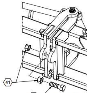
OPP. SIDE AT SWING HINGE
