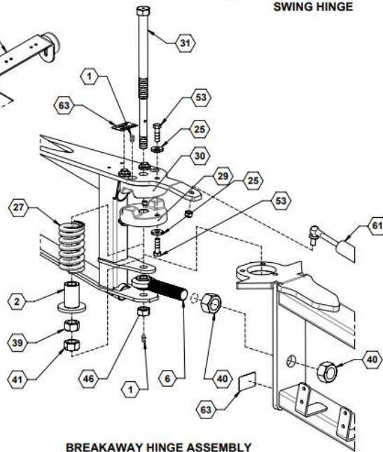
BREAKAWAY HINGE ASSEMBLY
