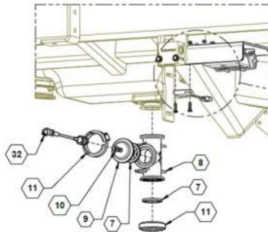
EXPLODED VIEW
