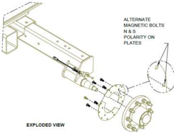
EXPLODED VIEW
