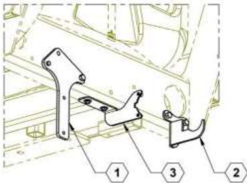
PLUMBING BRACKET ASSEMBLY
