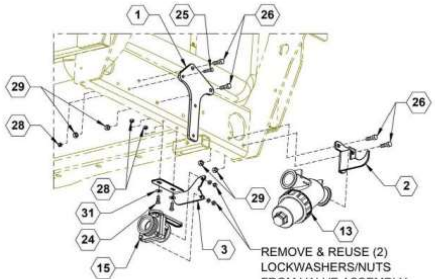
BRACKET ASSEMBLY EXPLODED
