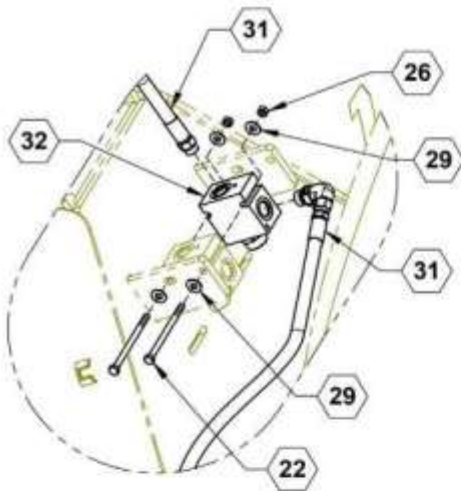
DETAIL AT FLOW REGULATOR
