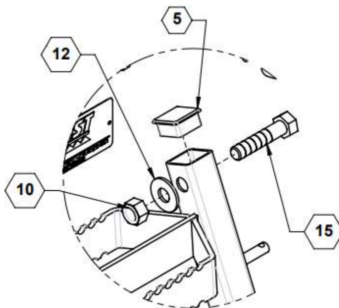
DETAIL B SCALE 1 : 4
