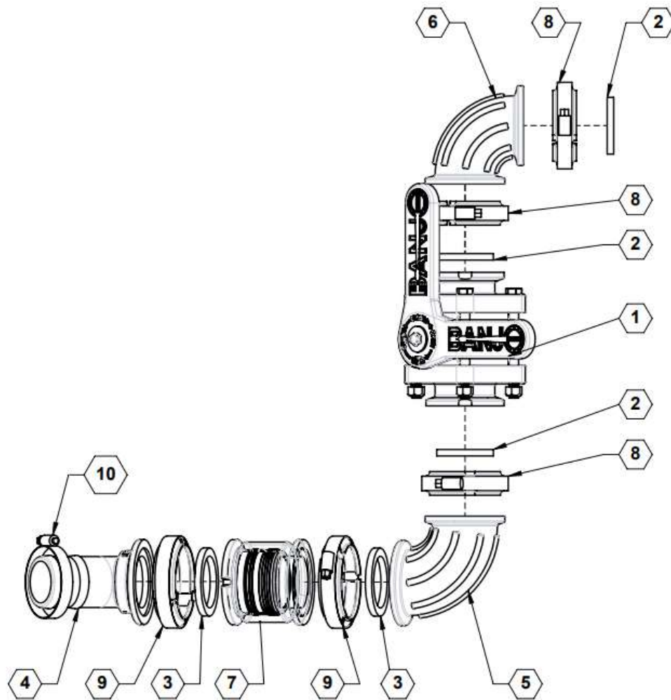
Parts List 90SARAE2: Distribution Bank End Takeoff
