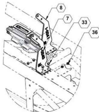
DETAIL D SCALE 1 : 8
