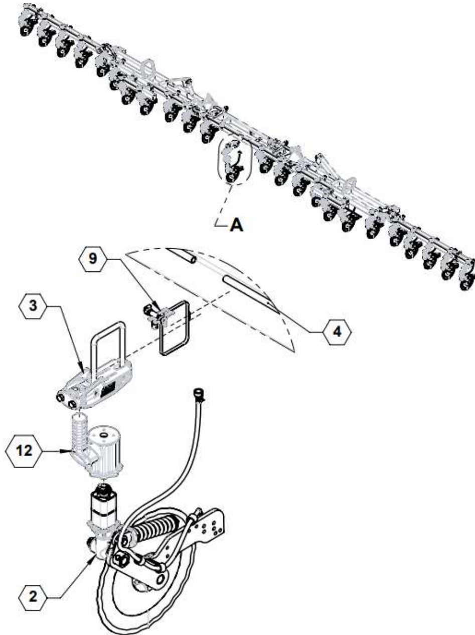
DETAIL A
