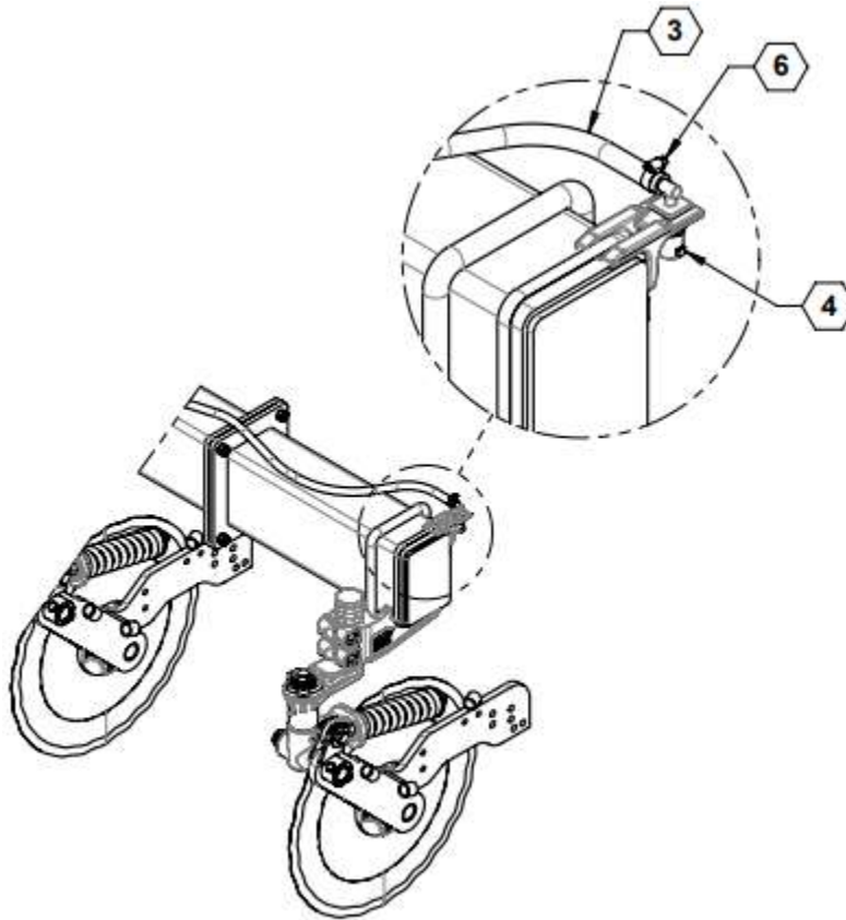
PARTIAL ASSEMBLY VIEW AT LEFT END OF TOOLBAR, RIGHT END SIMILAR
