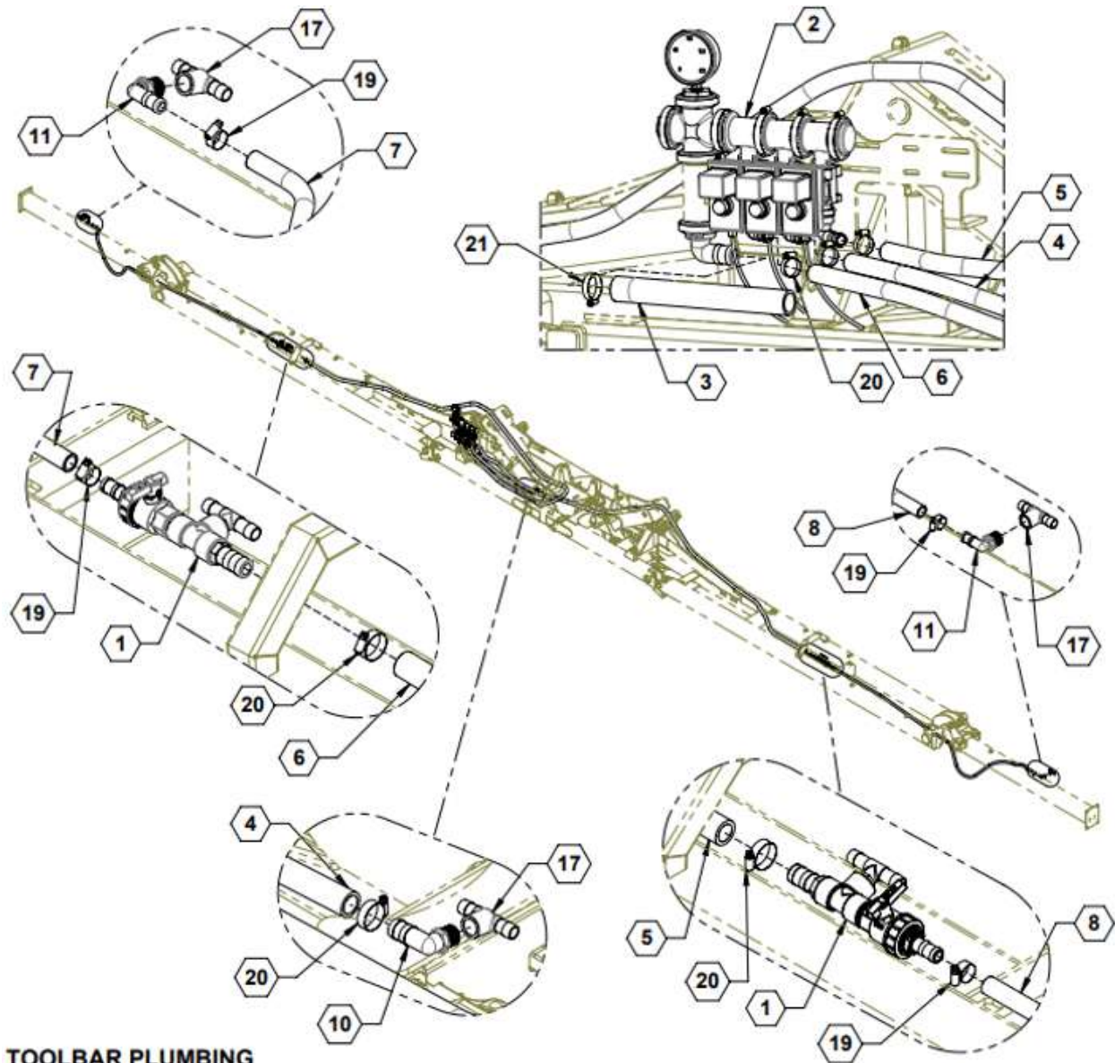
TOOLBAR PLUMBING
