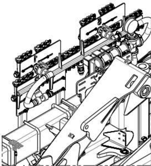
REAR VIEW OF WILGER MONITORS & ELECTRIC VALVES
