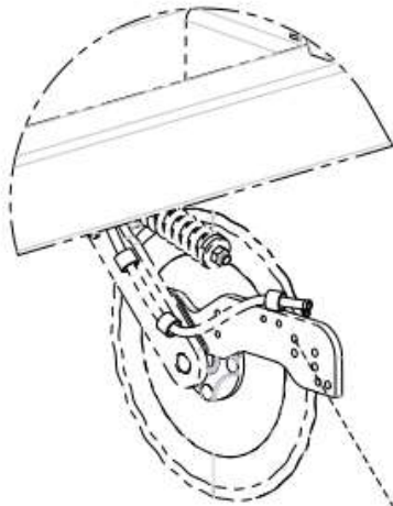
DETAIL B
